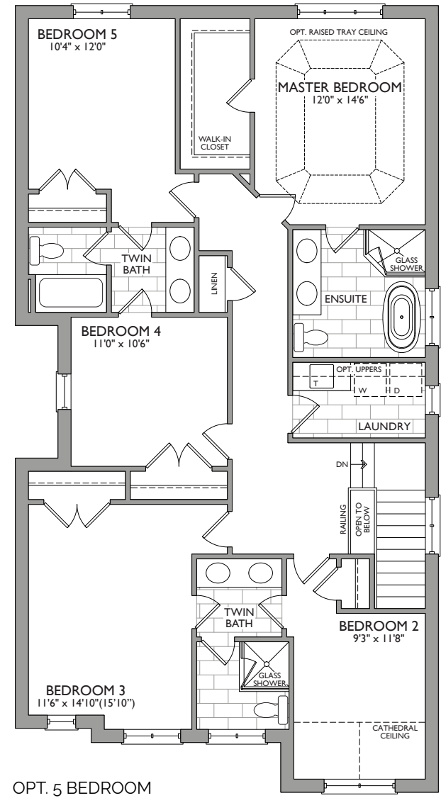
OPT. 5 BEDROOM SECOND FLOOR ELEV. A
