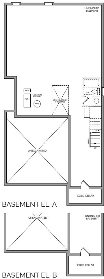
BASEMENT EL. B
